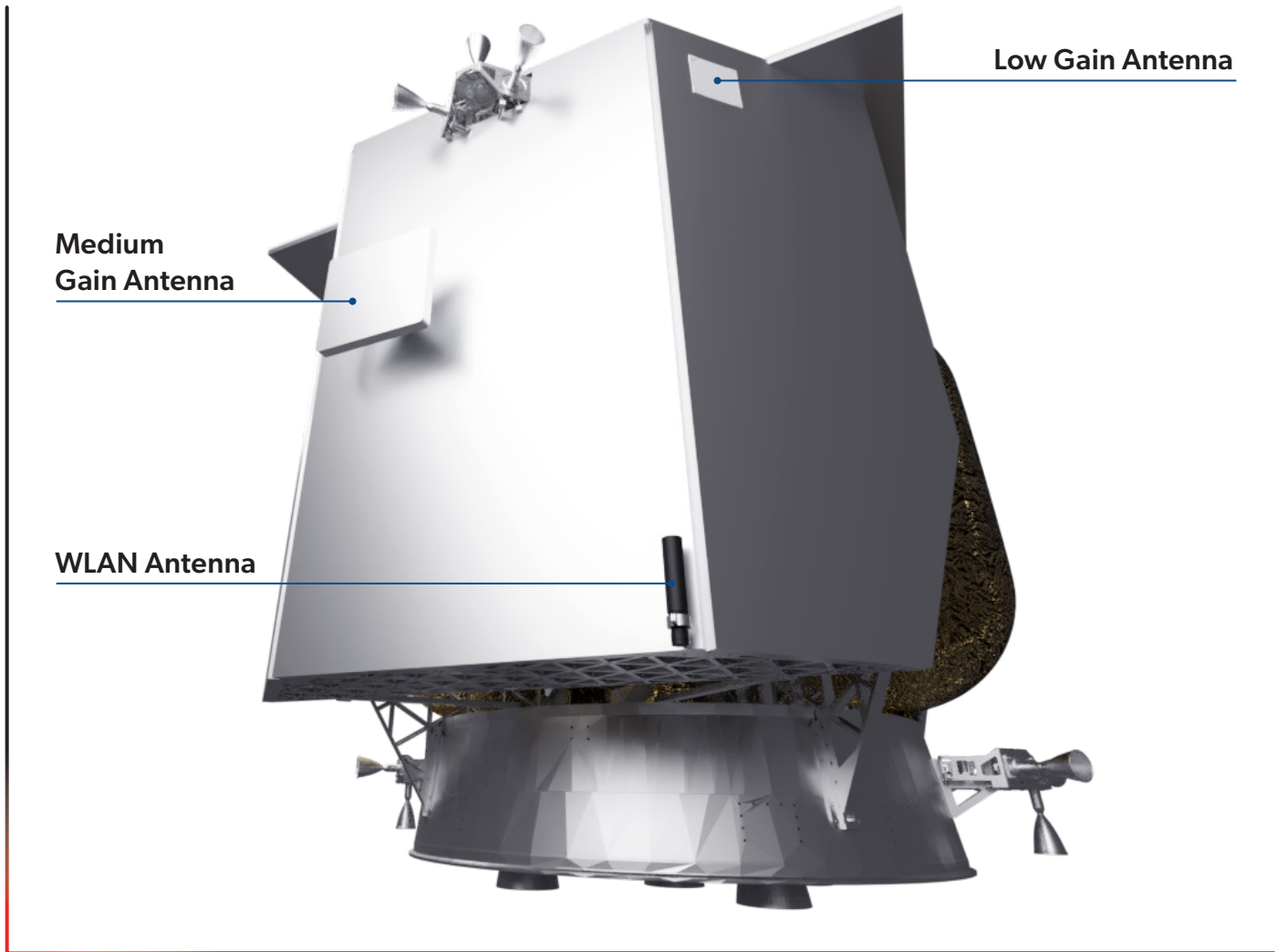
Peregrine Communications Bus
