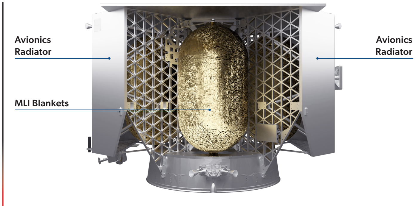
Peregrine Thermal Bus
