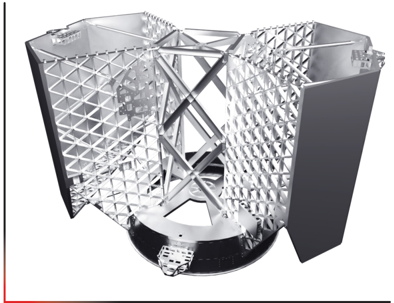
Peregrine Structural Bus
